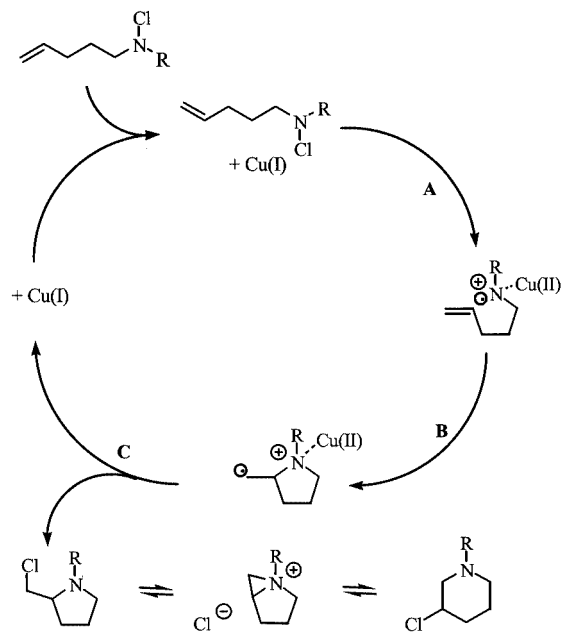
Figure 1. Catalytic cycle
