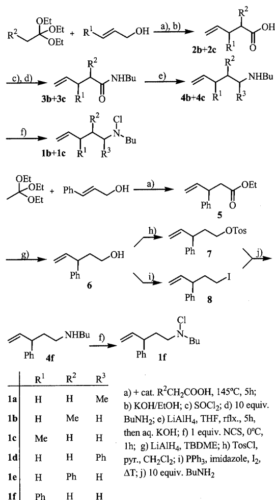
Figure 2. Synthesis of the chloroamines by a Johnson orthoester Claisen rearrangement
