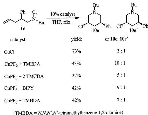
Figure 8. Diastereoselectivity in the cyclisation of chloroamine 1e
