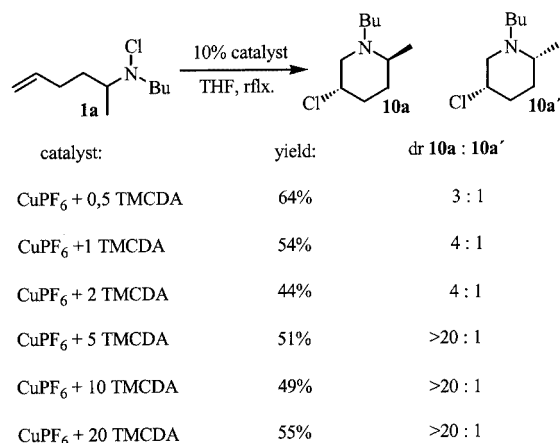
Figure 7. High diastereoselectivity with 5 equiv. of ligand
