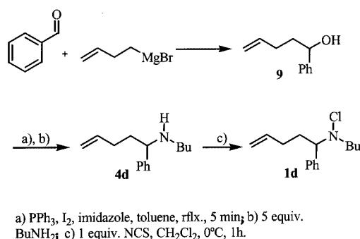
Figure 3. Synthesis of chloroamine 1d
