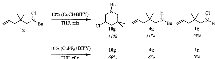
Figure 5. First experiments with addition of ligands
